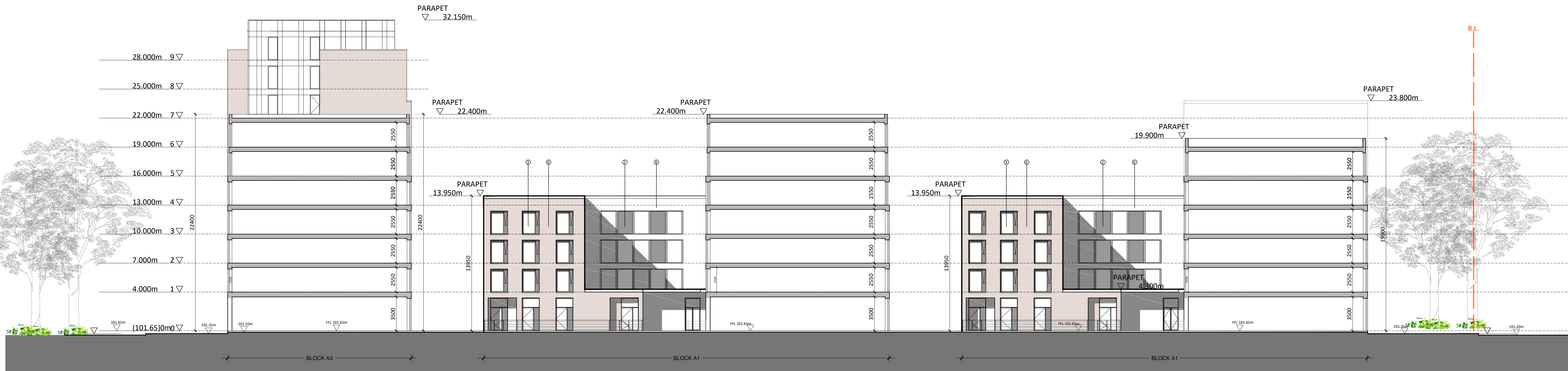
CONTEXTUAL ELEVATION SECTOR 1 - ELEVATION KK SCALE 1:200
