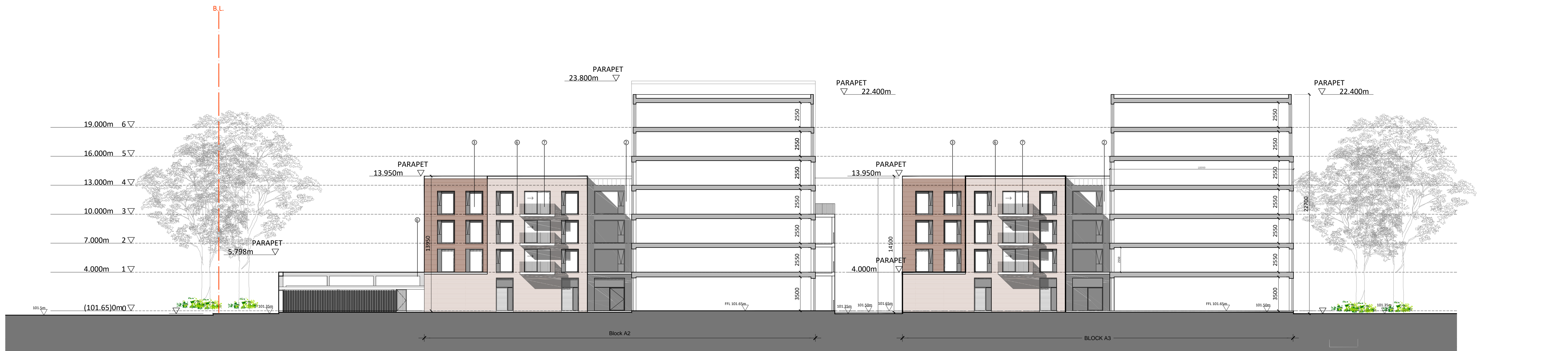
CONTEXTUAL ELEVATION SECTOR 1 - ELEVATION JJ SCALE 1:200
